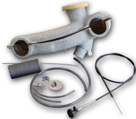
NAME: Intake airbox (a set) PART NO: A22L-03-150 WEIGHT: 0.73 kg
