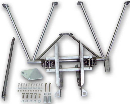
NAME: Engine mount (a set) PART NO: A22L-03-001 WEIGHT: 4.9 kg
