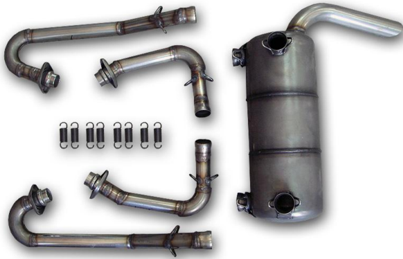
NAME: Exhaust system (80 hp, a set) PART NO: A22L-03-756 WEIGHT: 4.4 kg
